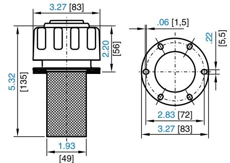
Type EB 80-10
